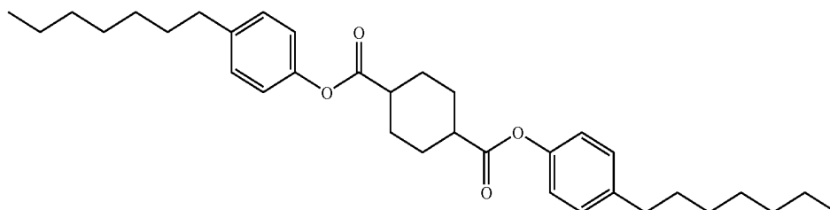
Structural Formula (A)
