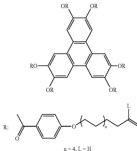
Structural Formula (F)
