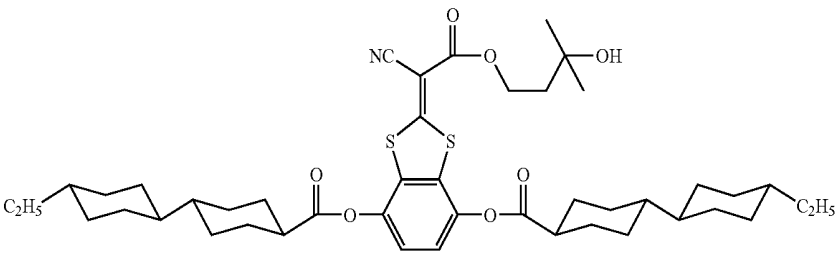
Structural Formula (G)
