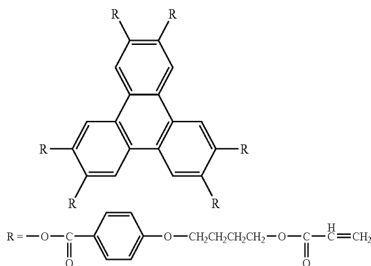
Discotic Liquid Crystal Molecule (I)
