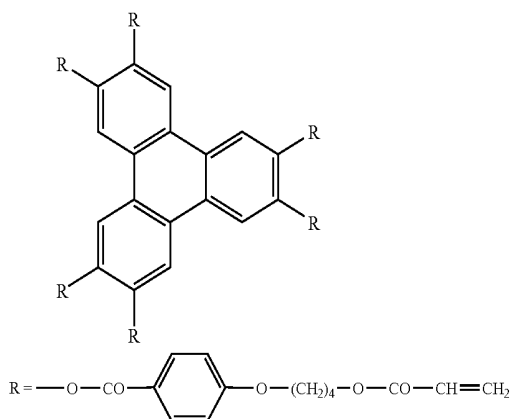
Discotic liquid crystal compound
