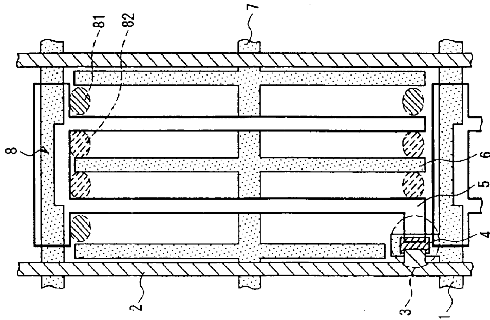
FIG. 9B (Termination Side)
