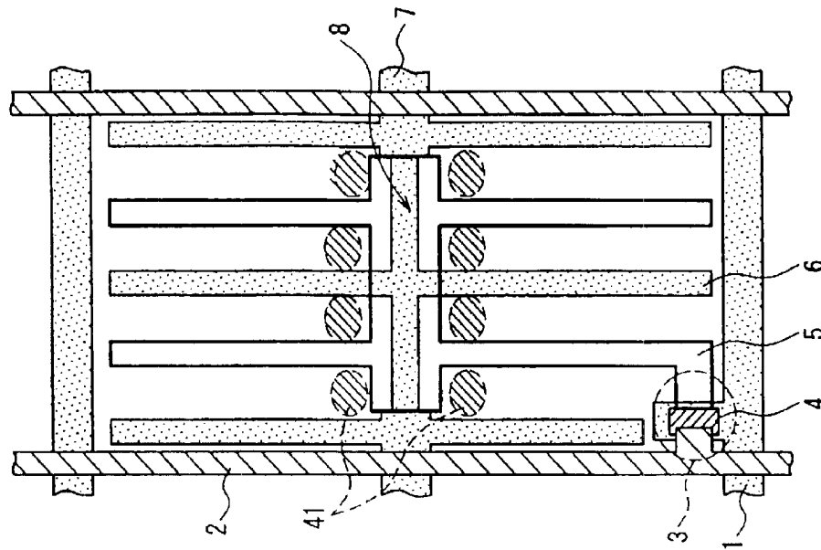
FIG. 4B (Termination Side)
