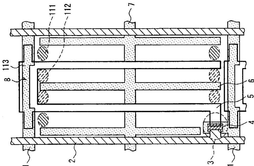
FIG. 11B (Termination Side)
