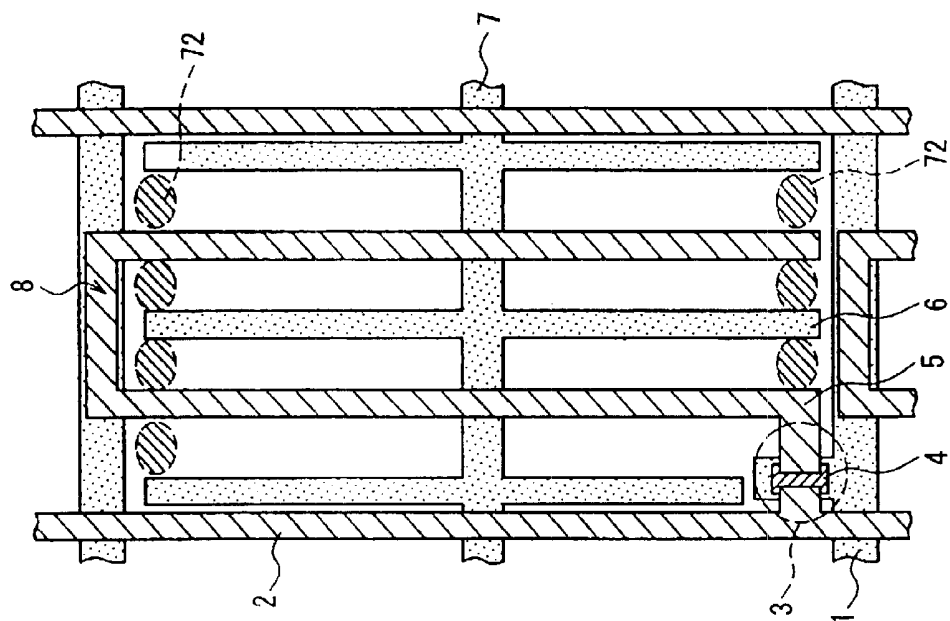
FIG. 7B (Termination Side)
