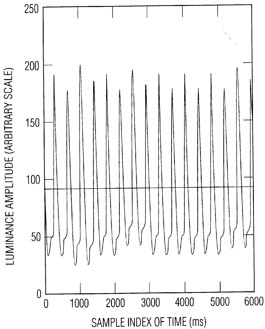
FIG. 4 PRIOR ART
