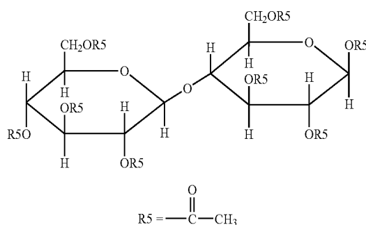
Compound 5
