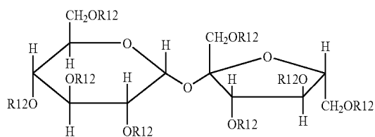
Compound 12
