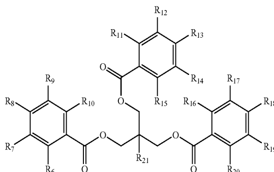
Formula (5)
