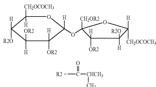
Compound 2
