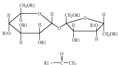
Compound 1
