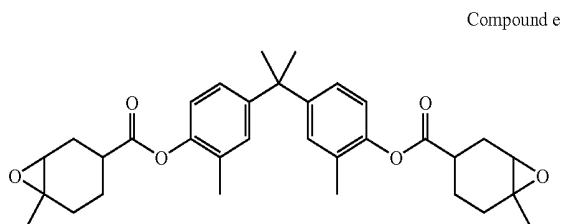
Compound e
