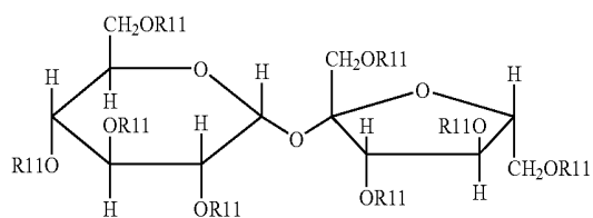
Compound 11
