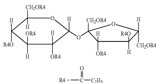
Compound 4
