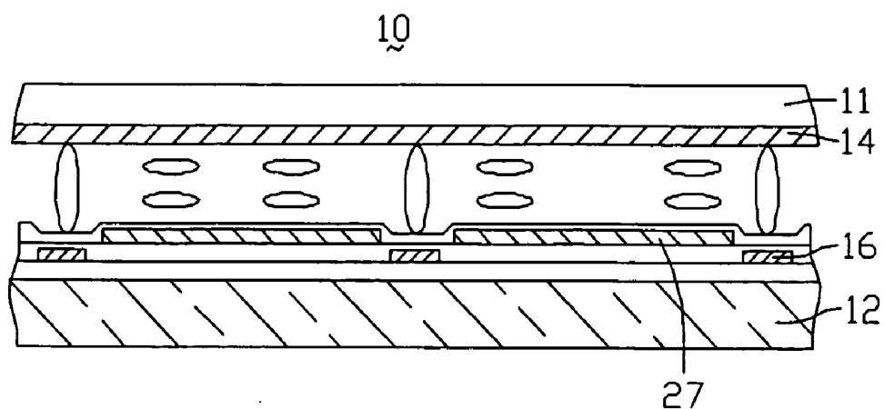
FIG. 11 (RELATED ART)
