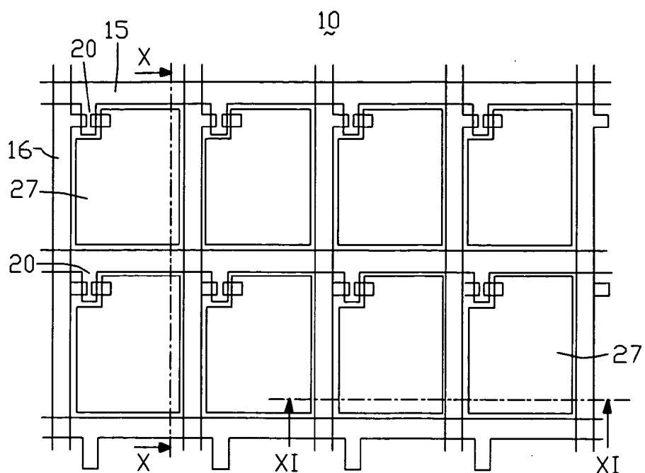
FIG. 9 (RELATED ART)
