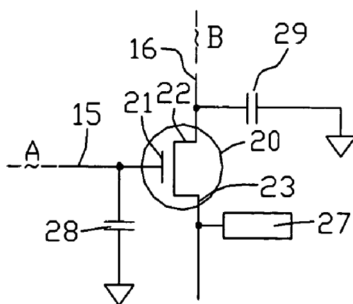
FIG. 12 (RELATED ART)
