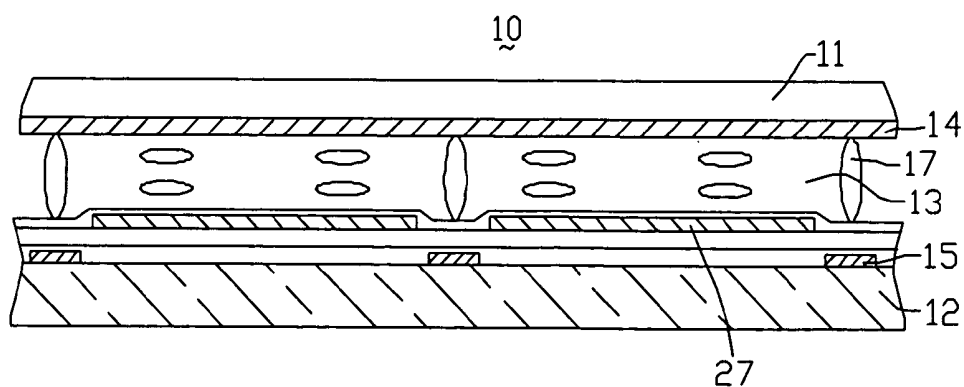
FIG. 10 (RELATED ART)
