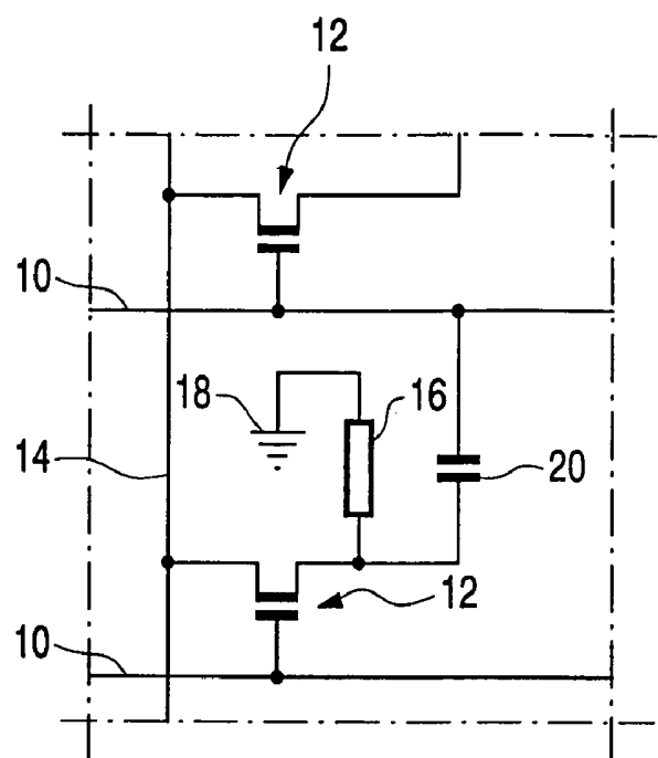
Fig.1 PRIOR ART
