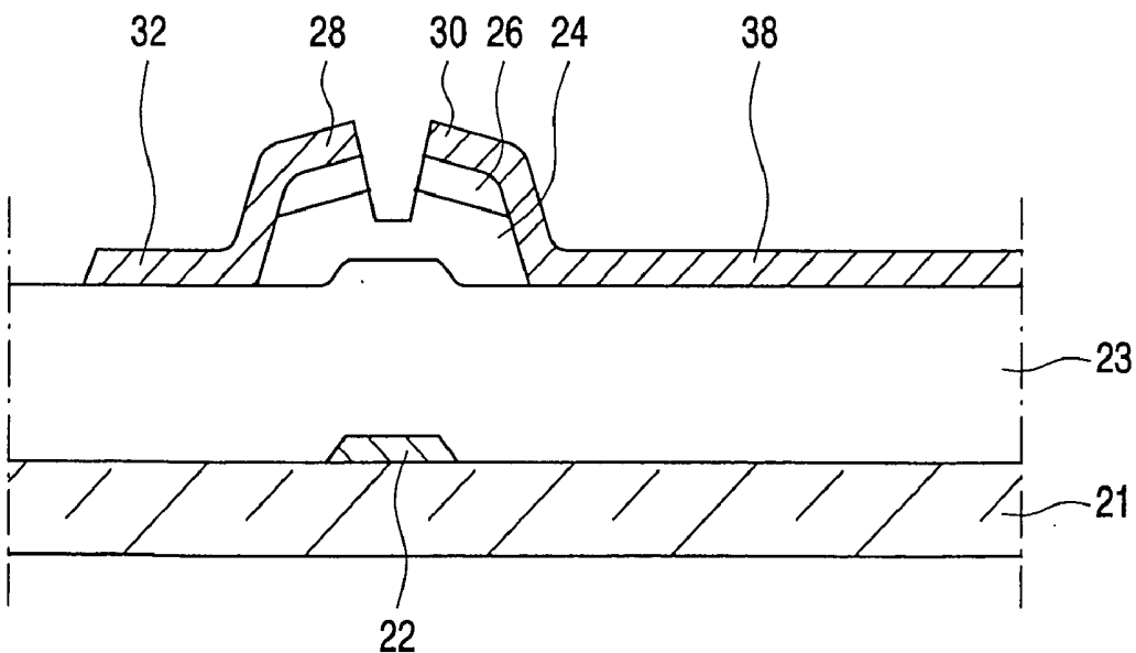
Fig.3 PRIOR ART
