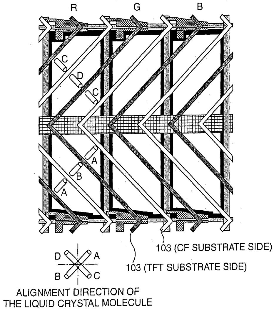
PIXEL STRUCTURE OF AN MVA LIQUID CRYSTAL DISPLAY (ONE PIXEL)
