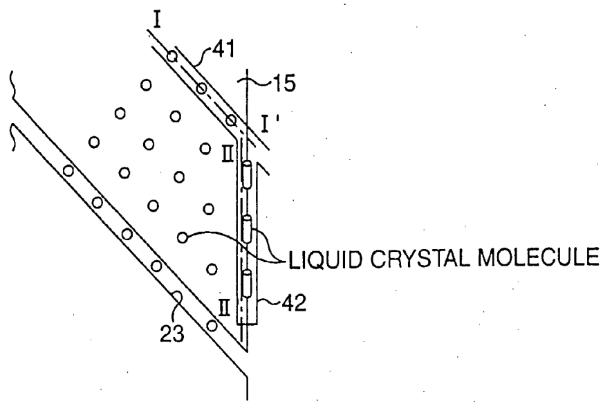
PLANE VIEW
