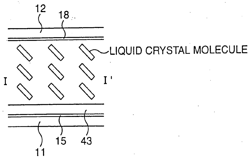
SECTIONAL VIEW
