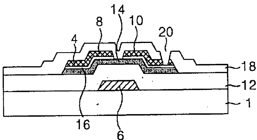
FIG. 3C RELATED ART
