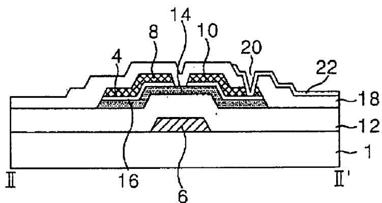
FIG. 2 RELATED ART
