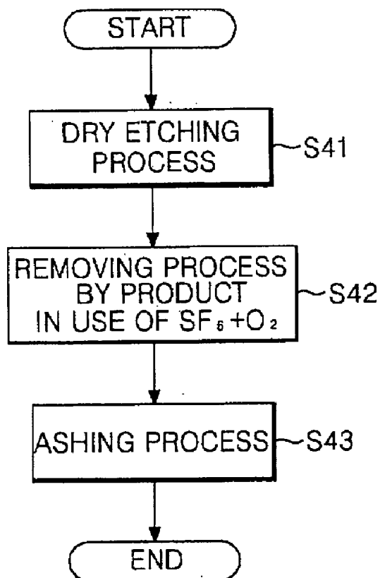
FIG. 4 RELATED ART
