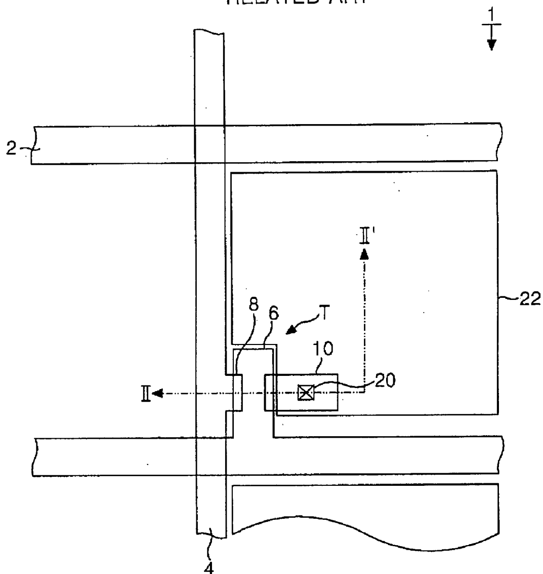
FIG. 1 RELATED ART
