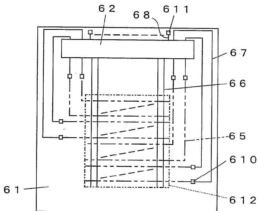
FIG. 20 PRIOR ART
