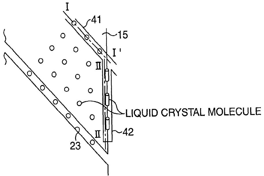
PLANE VIEW
