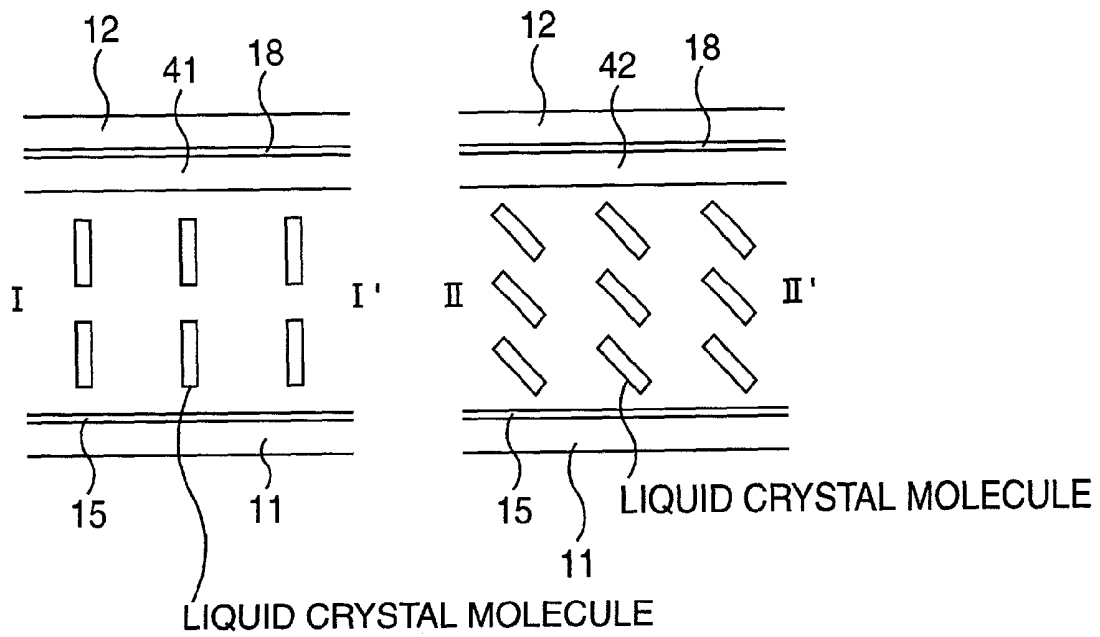
SECTIONAL VIEW
