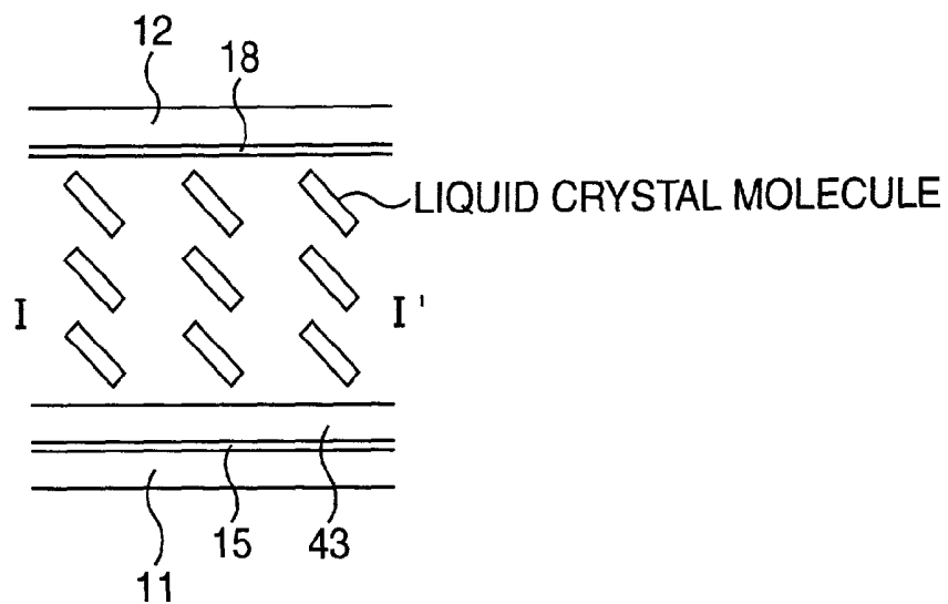
SECTIONAL VIEW
