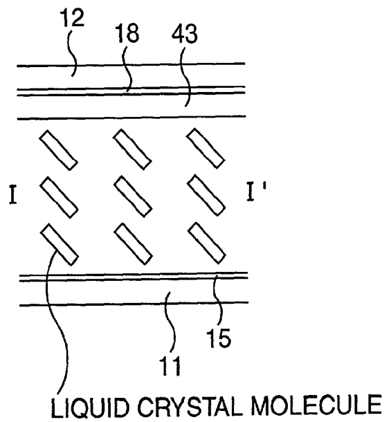
SECTIONAL VIEW
