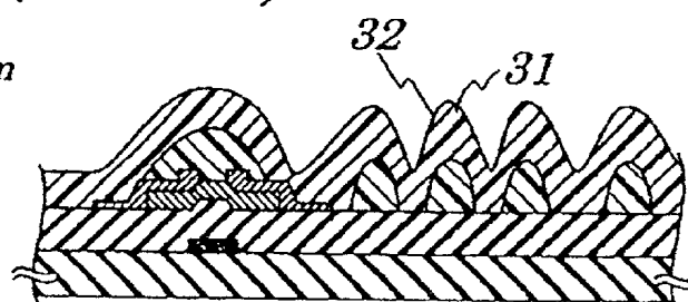
FIG.21I (PRIOR ART) forming contact region
