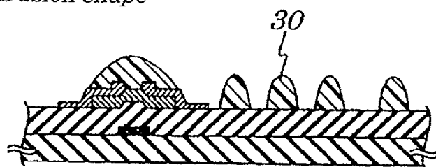
FIG.21G (PRIOR ART) smooth protrusion shape
