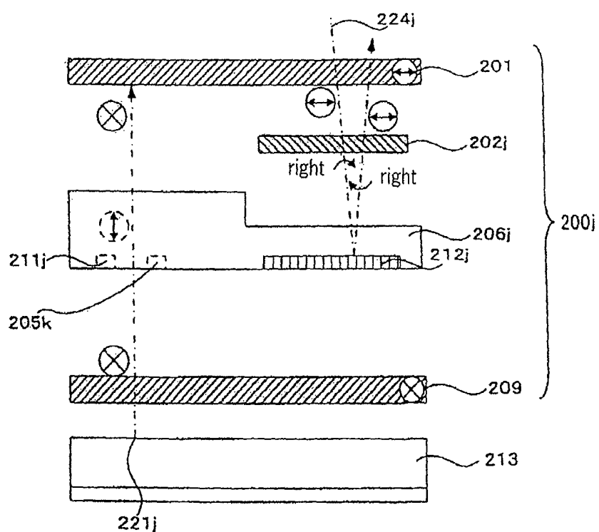
Fig.36B
