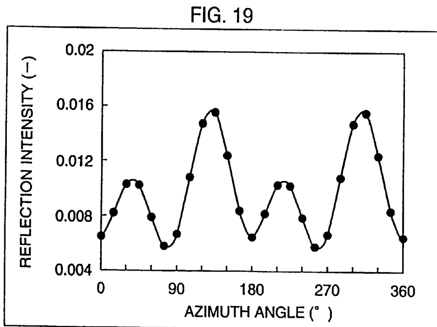
POLARIZING PLATE + \lambda/4 AZIMUTH ANGLE CHARACTERISTICS (1) (30° INCIDENCE)
