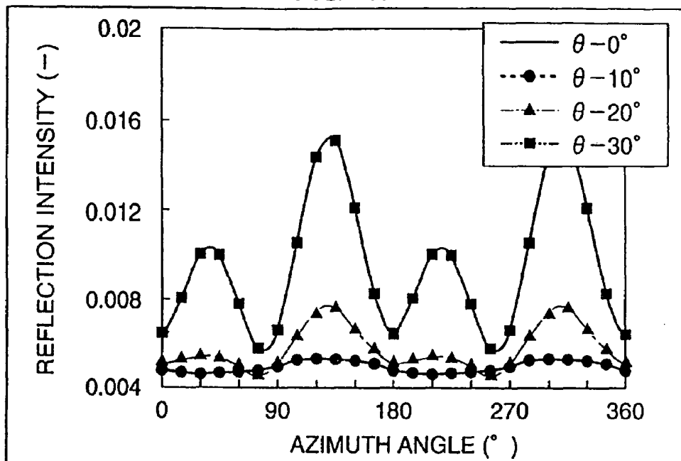
POLARIZING PLATE + \lambda/4 PLATE AZIMUTH ANGLE CHARACTERISTICS (2) (0-30° INCIDENCE)
