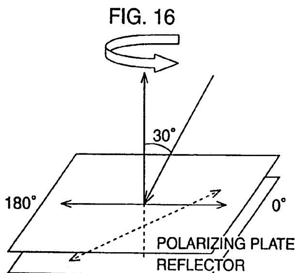
CONFIGURATION OF SINGLE POLARIZING PLATE AND MEASUREMENT METHOD
