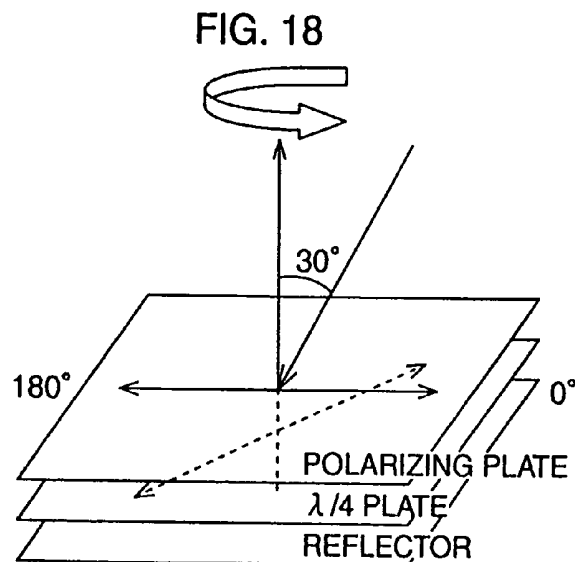
CONFIGURATION OF POLARIZING PLATE + \lambda/4 AND MEASUREMENT METHOD
