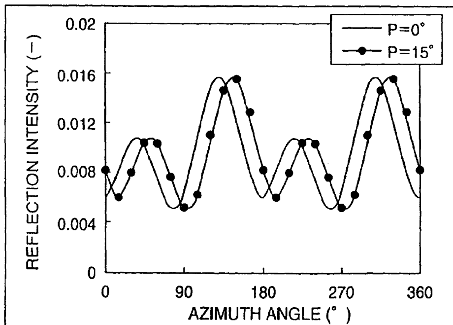
POLARIZING PLATE + \lambda/4 PLATE AZIMUTH ANGLE CHARACTERISTICS (3) (30° INCIDENCE)
