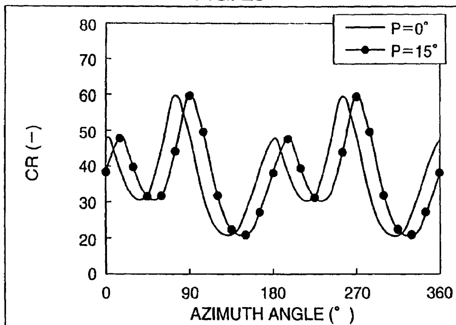
POLARIZING PLATE + \lambda/4 PLATE AZIMUTH ANGLE CHARACTERISTICS (4) (30° INCIDENCE)
