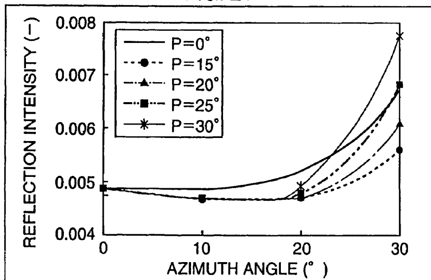
POLARIZING PLATE + \lambda/4 PLATE INCIDENT ANGLE CHARACTERISTICS (1) (270° AZIMUTH)
