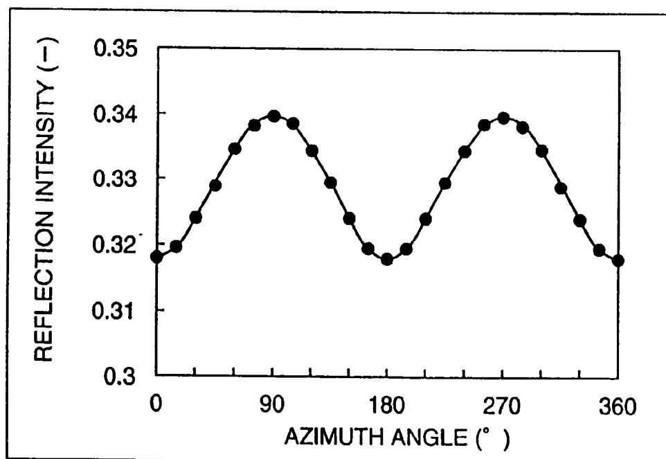
AZIMUTH ANGLE CHARACTERISTICS OF SINGLE POLARIZING PLATE (30° INCIDENCE)
