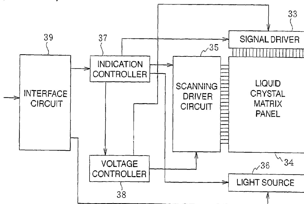
FIG. 19 (PRIOR ART)
