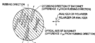
ALIGNMENT LAYERS, CONTACT ANGLES, EXTENDING DIRECTIONS AND OPTICAL AXES OF BATONNET (ANGLES SHIFTED FROM RUBBING DIRECTION)
