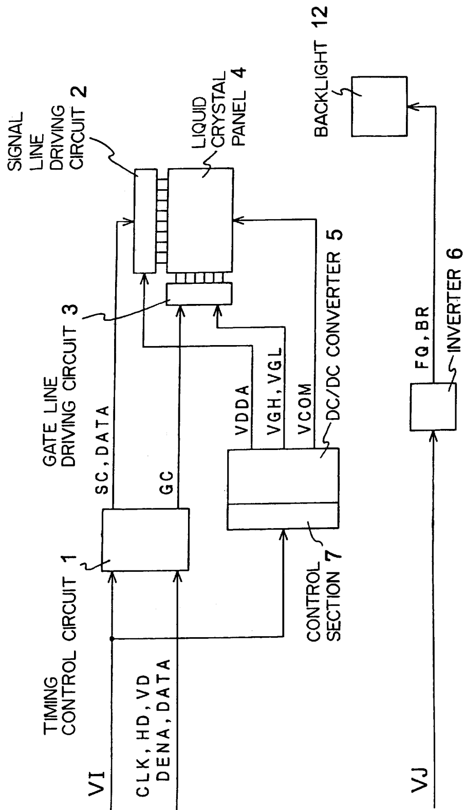
FIG. 3 BACKGROUND ART
