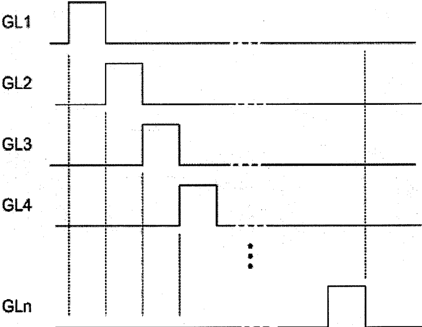
FIG. 3 (Related Art)
