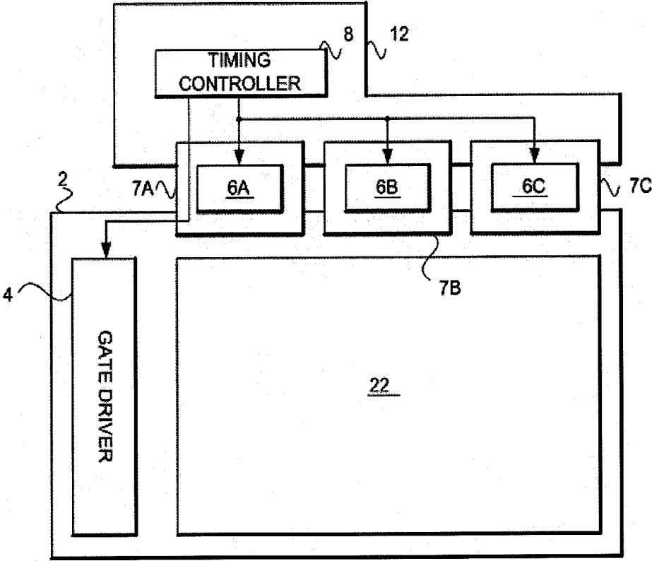
FIG. 1 (Related Art)
