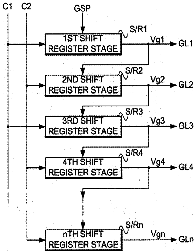
FIG. 2 (Related Art)
