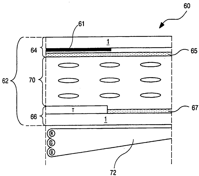
FIG. 2 (RELATED ART)
