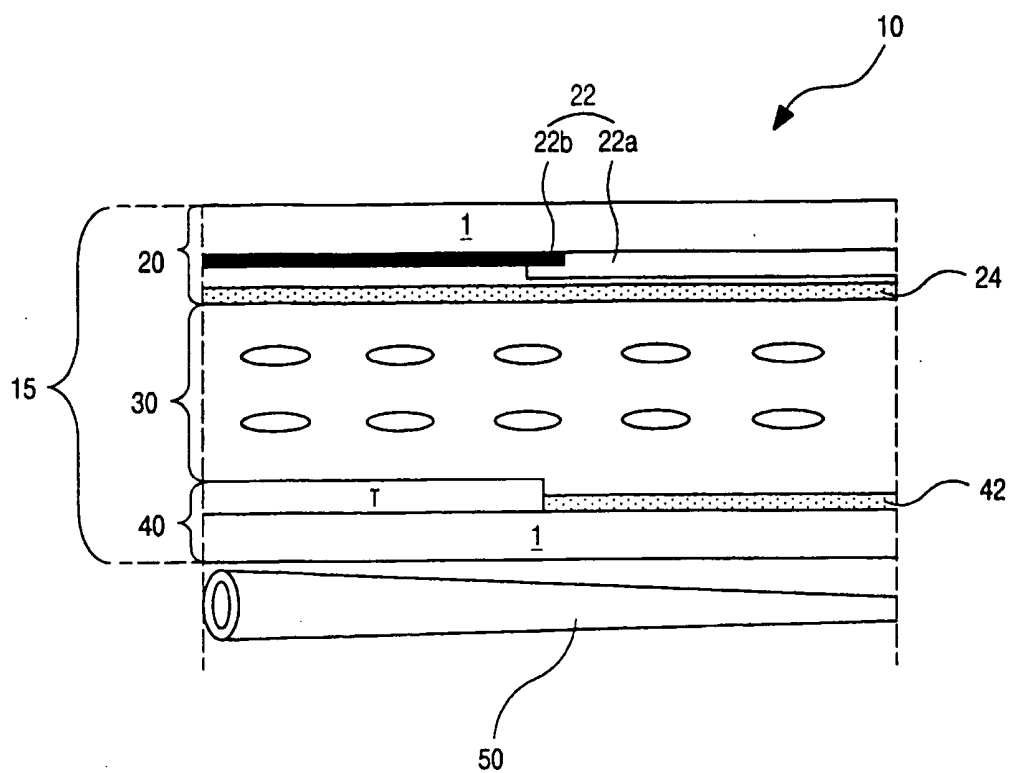
FIG. 1 (RELATED ART)
