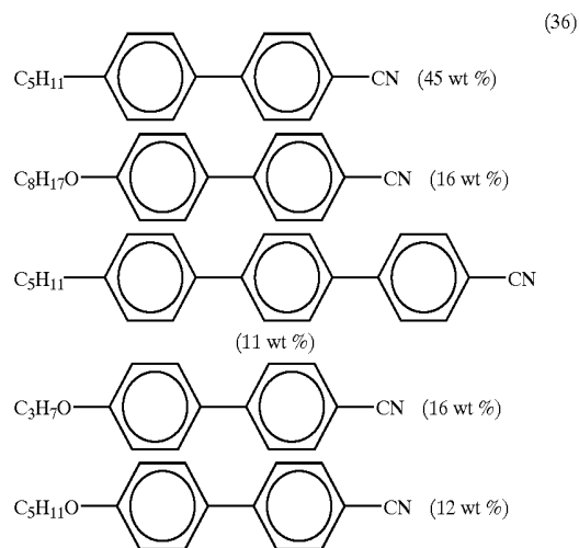
E8: Mixture of the Foregoing Five Kinds of Liquid Crystal
