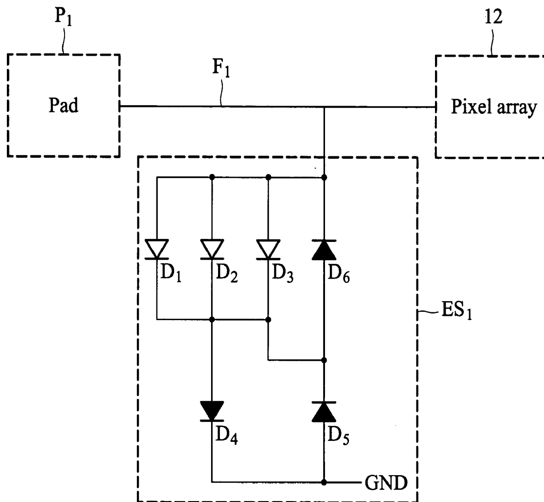
FIG. 2 (RELATED ART)
