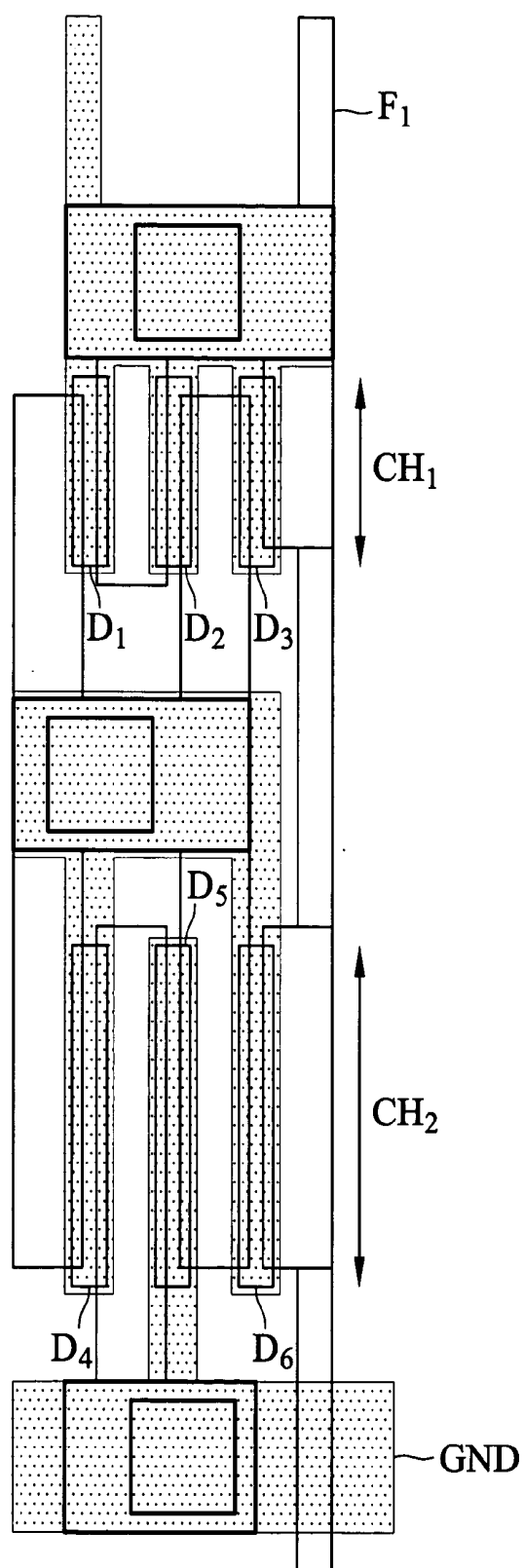
FIG. 3 (RELATED ART)
