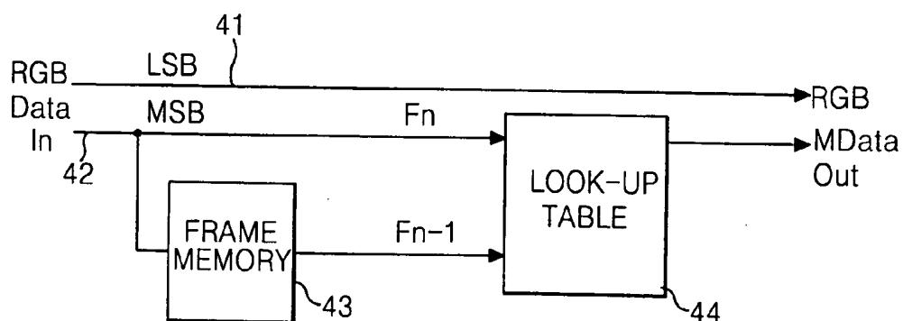
FIG. 4 CONVENTIONAL ART
