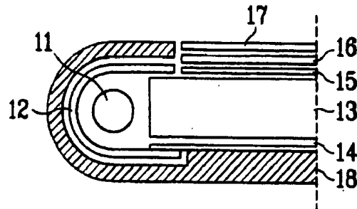
FIG. 3 Related Art
