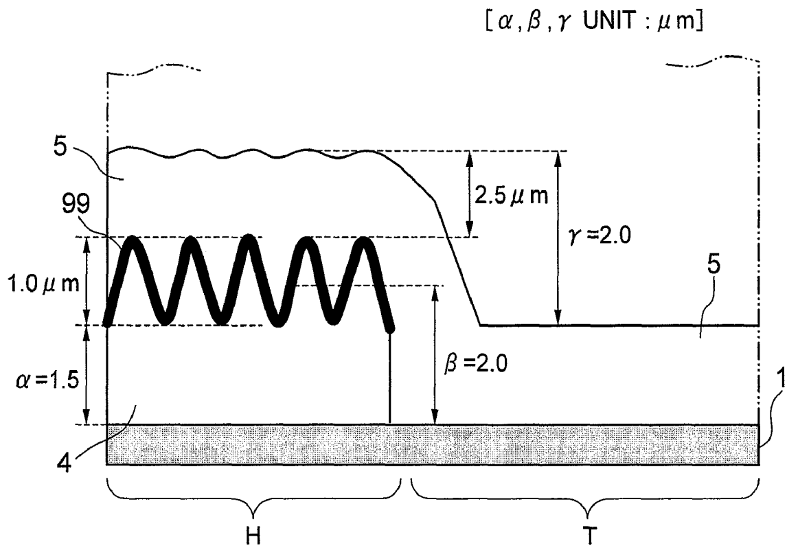
WITH TRANSMISSIVE PART FLATTENING FILM
