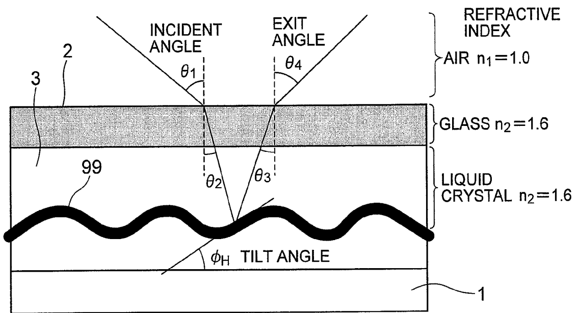
RELATION BETWEEN INCIDENT ANGLE/EXIT ANGLE AND TILT ANGLE
