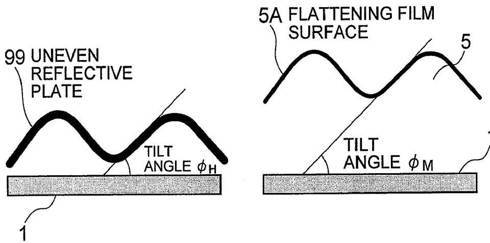
DEFINITION OF TILT ANGLE
