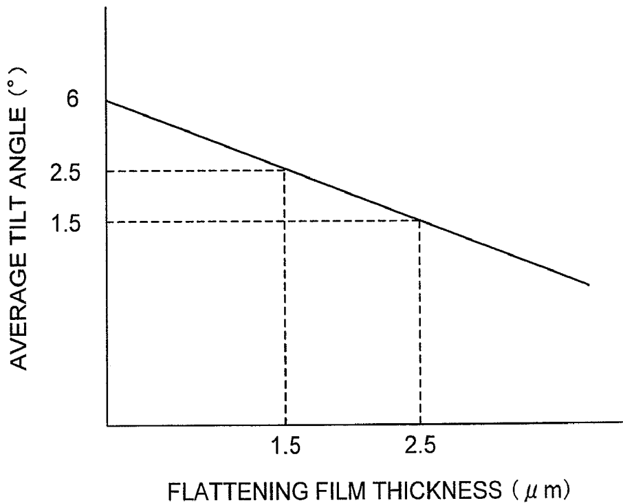
GRAPH OF RELATION BETWEEN FLATTENING FILM THICKNESS AND AVERAGE TILT ANGLE OF FLATTENING FILM SURFACE
