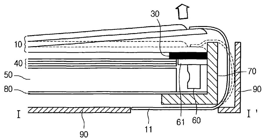
Fig. 2(Related Art)
