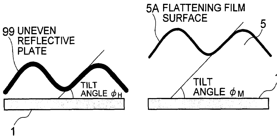
DEFINITION OF TILT ANGLE
