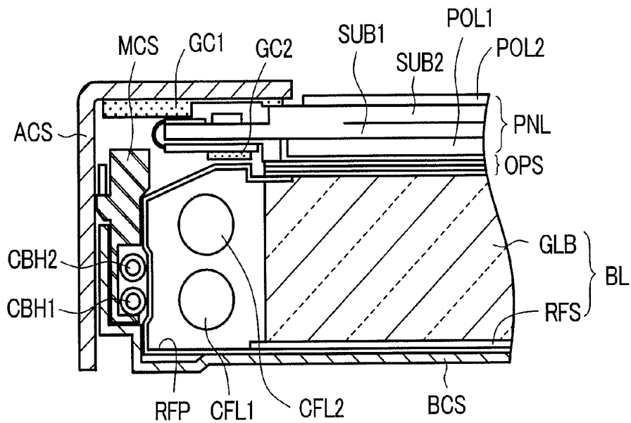
FIG. 9 (Prior Art)
