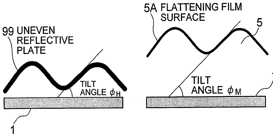
DEFINITION OF TILT ANGLE
