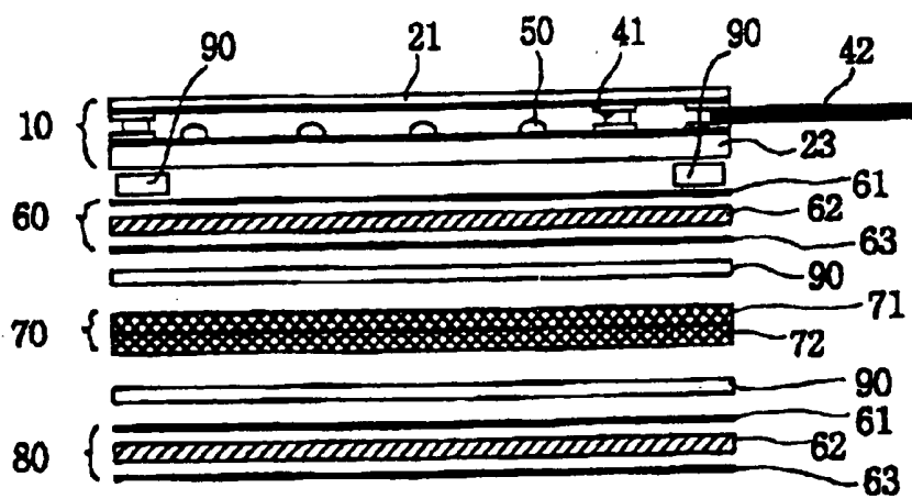
FIG. 2 (Prior Art)
