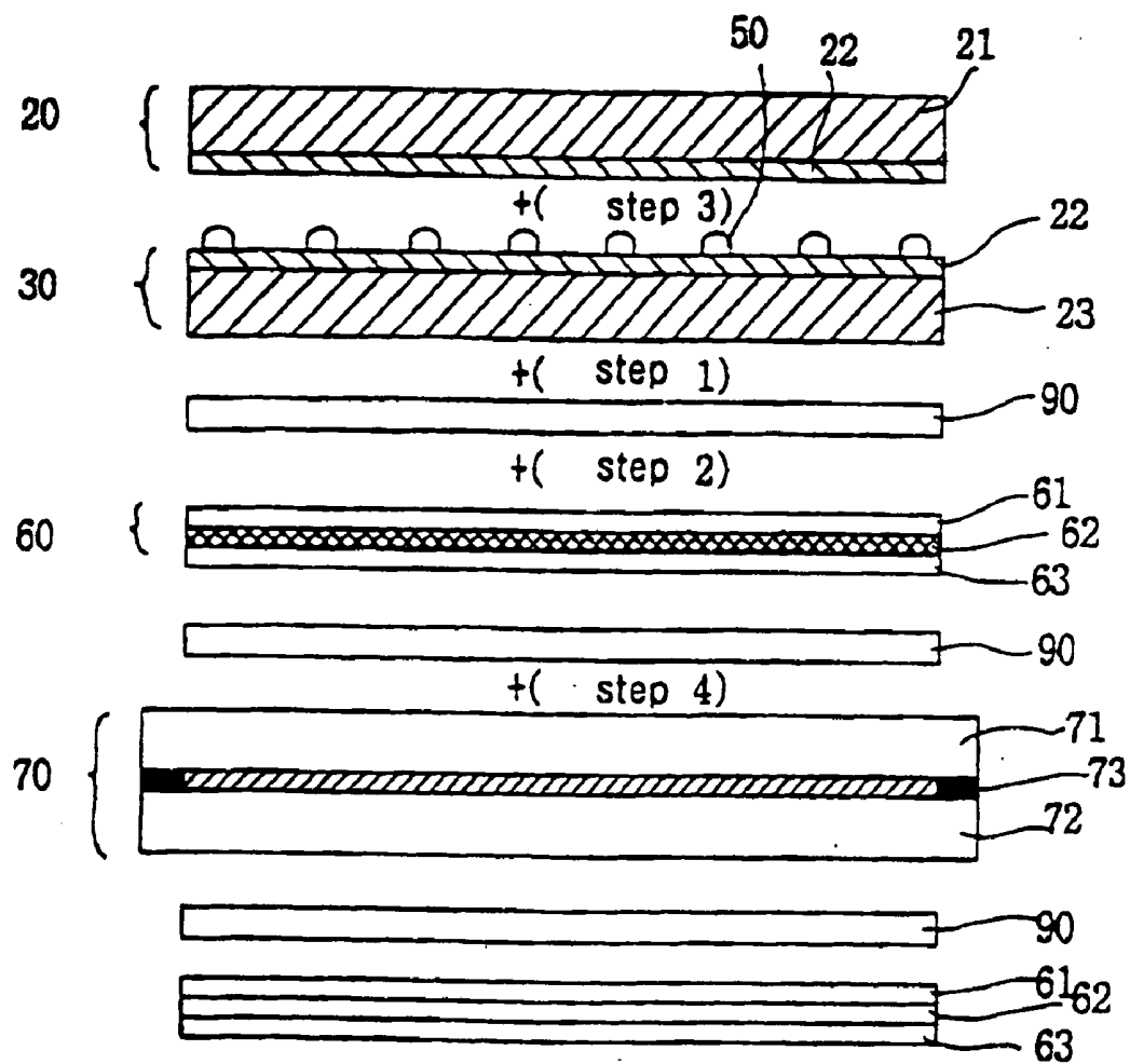
FIG. 5 (Prior Art)
