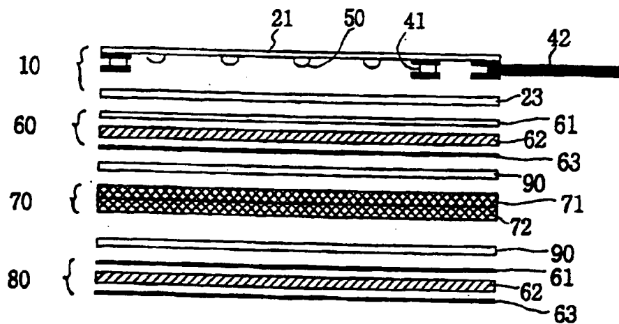
FIG. 4 (Prior Art)
