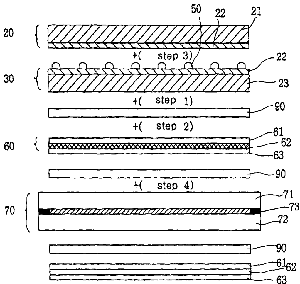
FIG. 5 (Prior Art)
