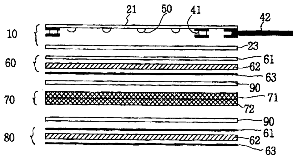
FIG. 4 (Prior Art)
