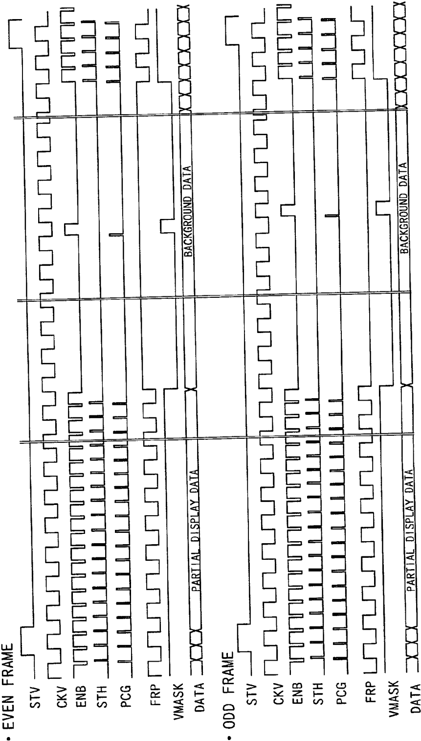
TIMING CHART IN PARTIAL DISPLAY (DRIVING METHOD 3 )
