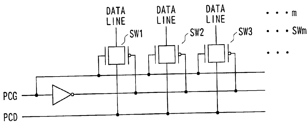
230 : PRE-CHARGE DRIVER
