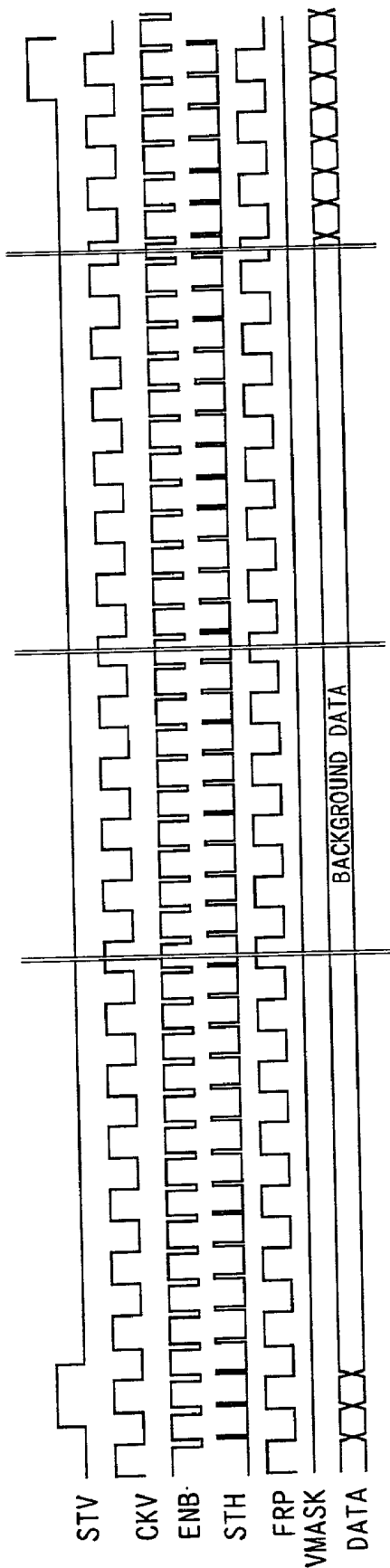
TIMING CHART IN BACKGROUND DISPLAY
