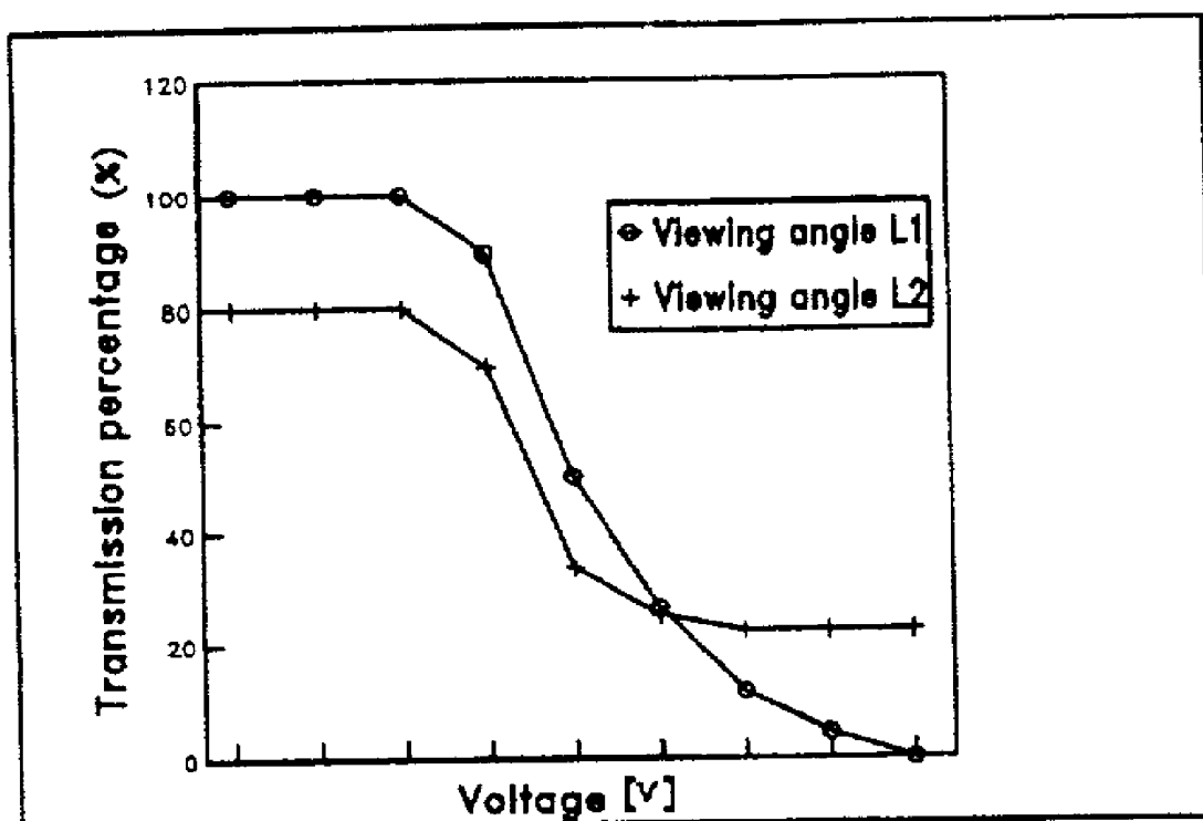
Viewing angle characteristic of two-domain LCD
