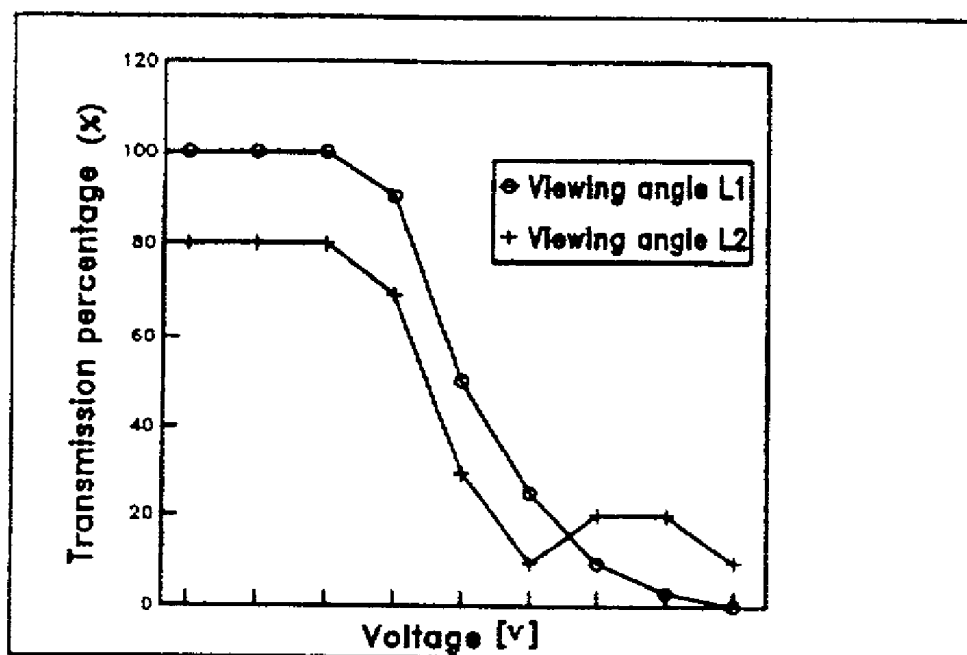
Viewing angle characteristic of single-domain LCD (reverse tilt)
