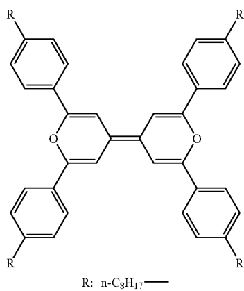
[Formula 12]
