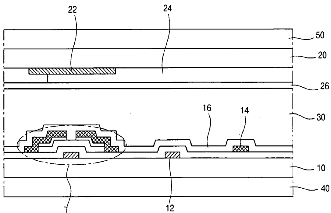
FIG. 1 RELATED ART
