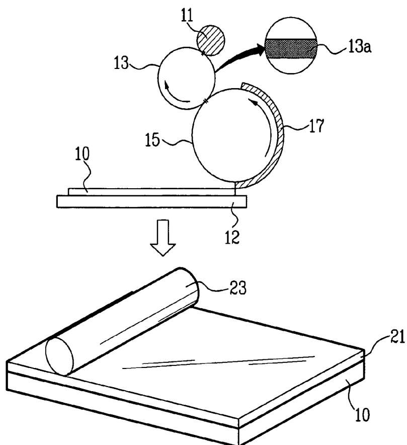
FIG.2 Related Art
