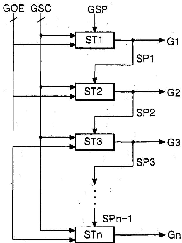
FIG. 4 RELATED ART
