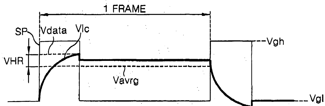
FIG. 4 RELATED ART
