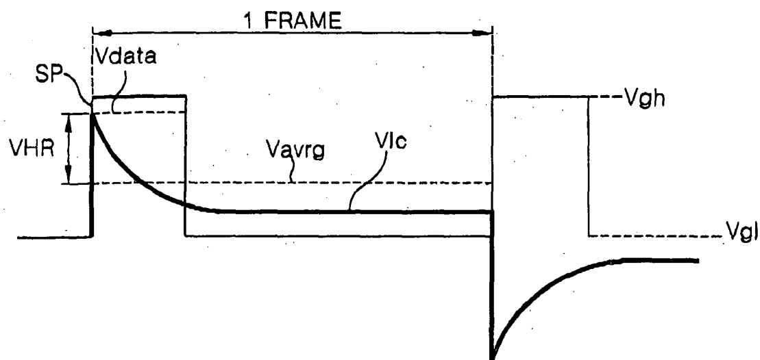
FIG. 10 RELATED ART
