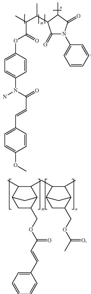
Chemical formula 3
