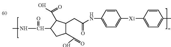
Chemical formula 6
