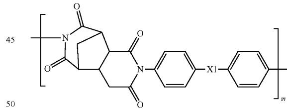
Chemical formula 7
