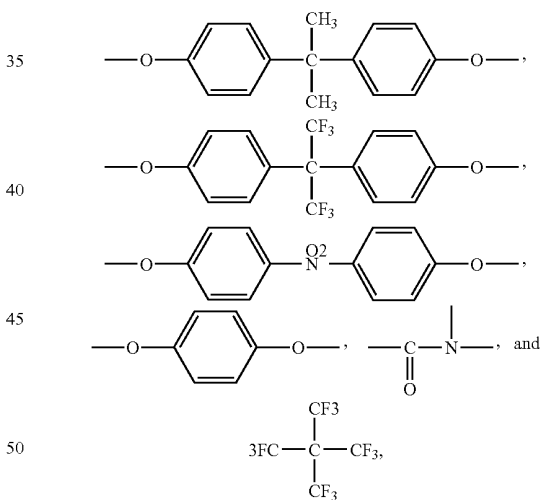
Chemical formula 3
