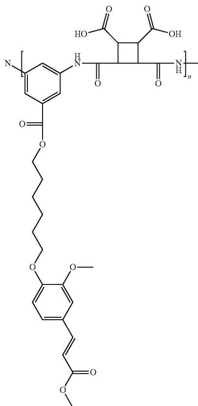
Chemical formula 4
