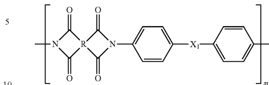
Chemical formula 5
