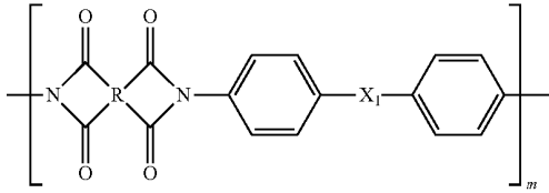
Chemical formula 5
