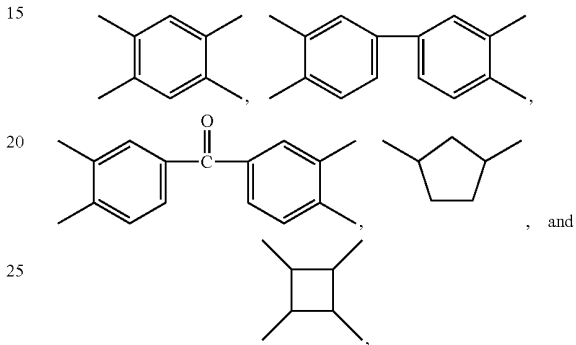
Chemical formula 2
