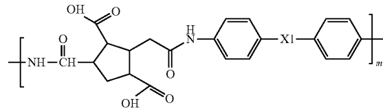
Chemical formula 6
