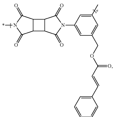
Chemical formula 2
