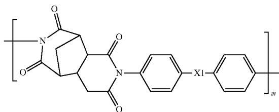
Chemical formula 7
