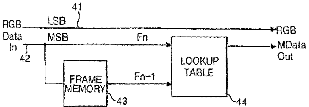
FIG. 4 RELATED ART
