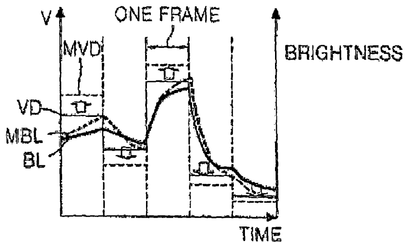
FIG. 2 RELATED ART
