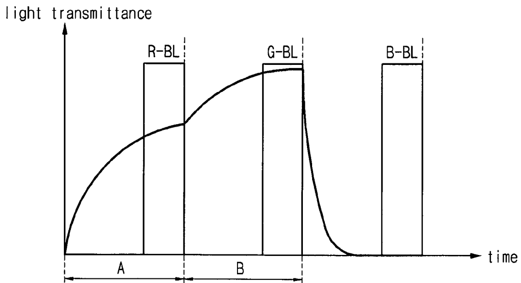
FIG. 2 RELATED ART
