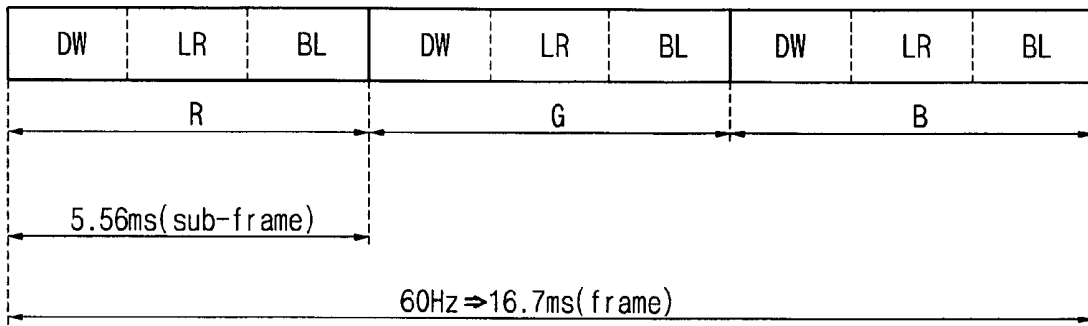
FIG. 1 RELATED ART
