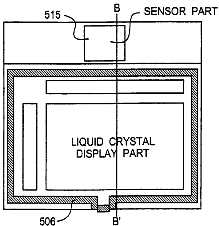
PLAN VIEW
