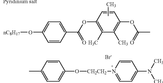
Pyridinium salt
