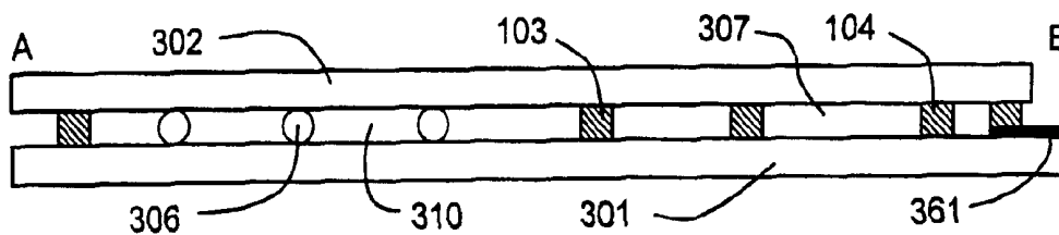
CROSS SECTIONAL VIEW TAKEN ON LINE A - B
