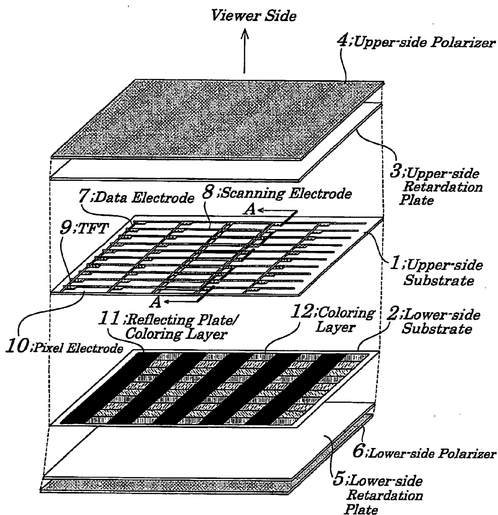
FIG. 17 (PRIOR ART)
