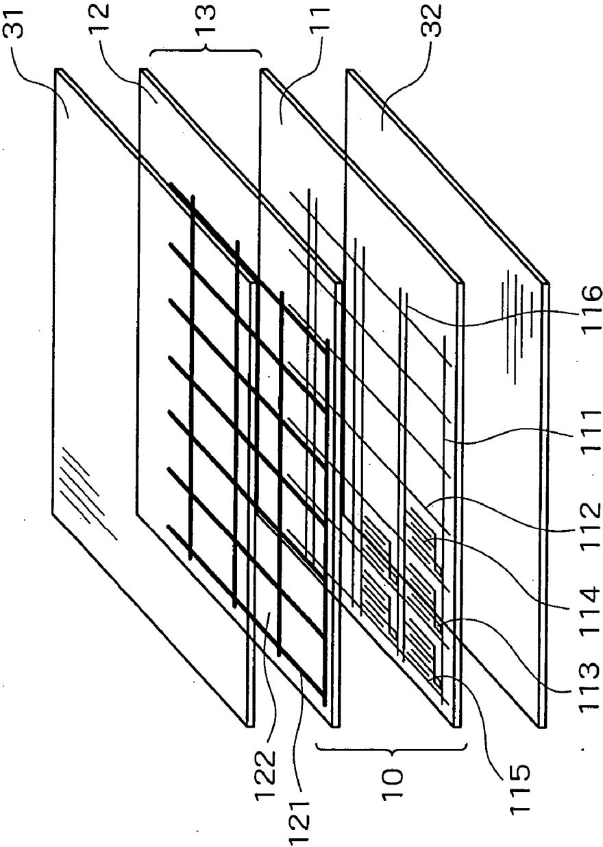
FIG. 1 (PRIOR ART)
