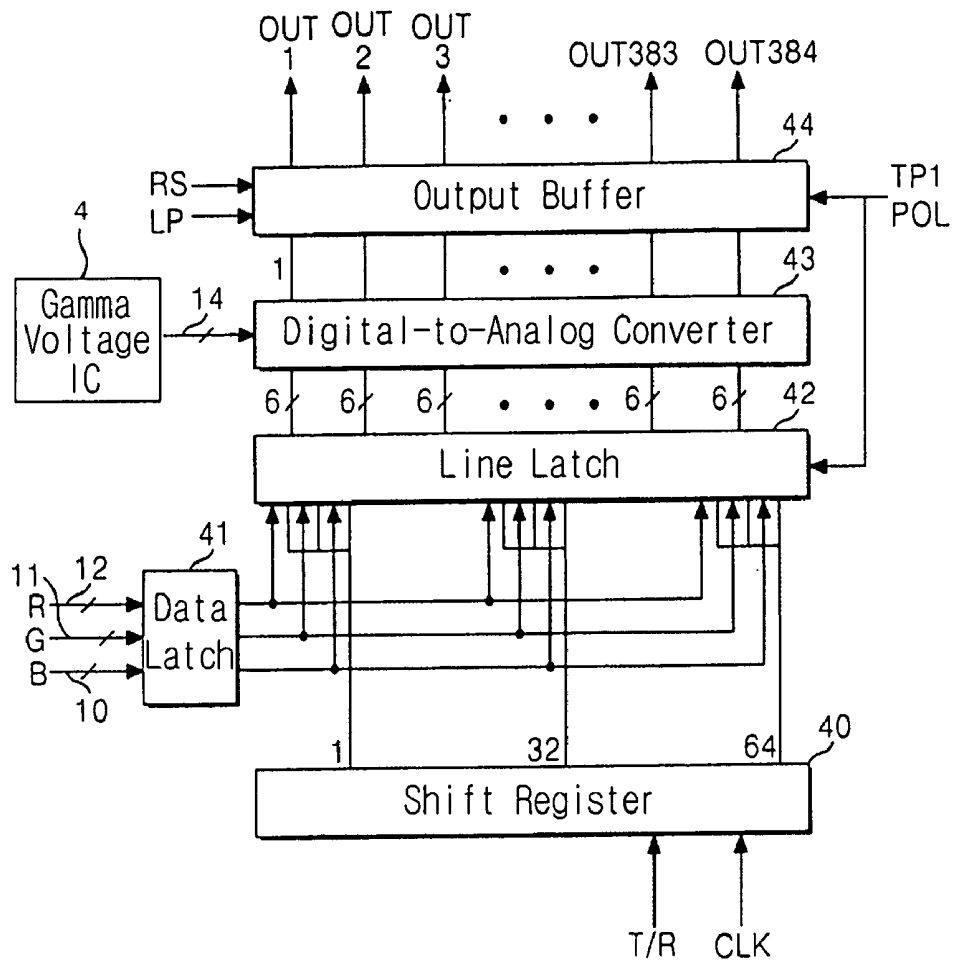
Fig.2 Related Art
