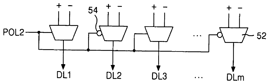
FIG. 7 RELATED ART
