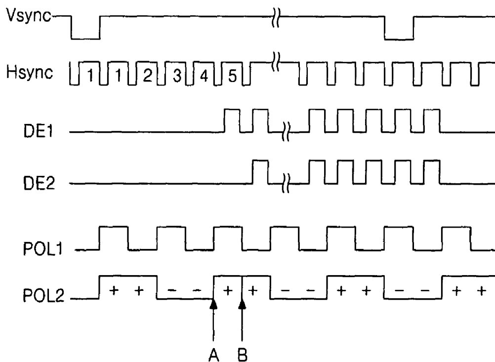
FIG. 6 RELATED ART
