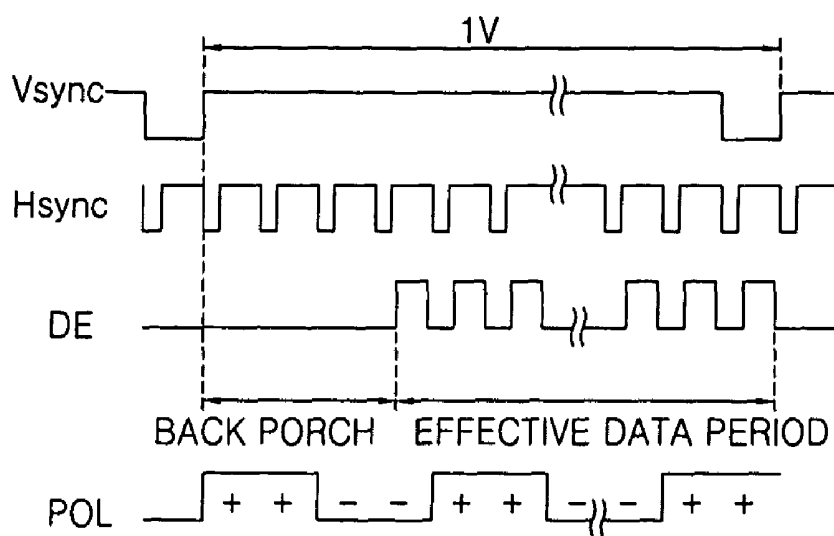
FIG. 4 RELATED ART
