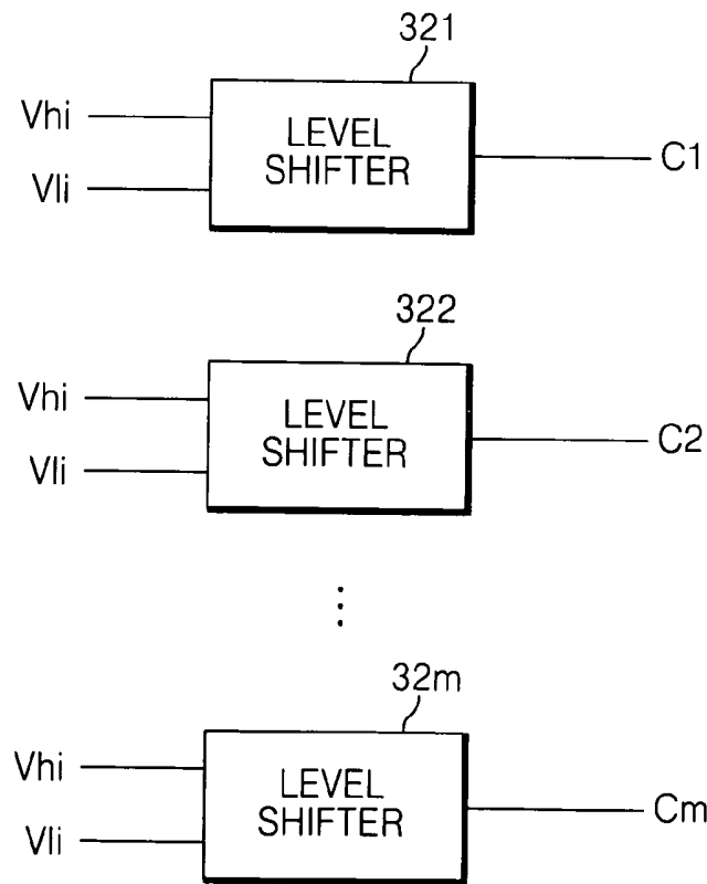
FIG.4 RELATED ART
