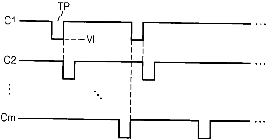
FIG.3 RELATED ART
