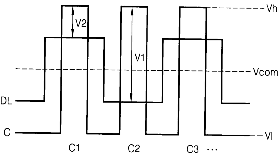
FIG. 10 RELATED ART
