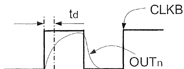
Fig. 1c (PRIOR ART)
