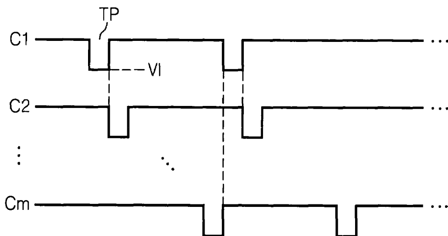
FIG. 3 RELATED ART
