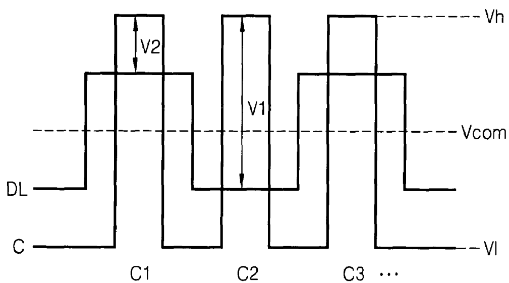
FIG. 10 RELATED ART
