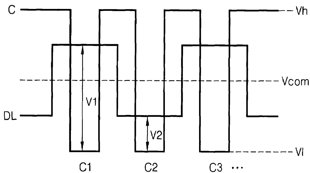
FIG. 9 RELATED ART
