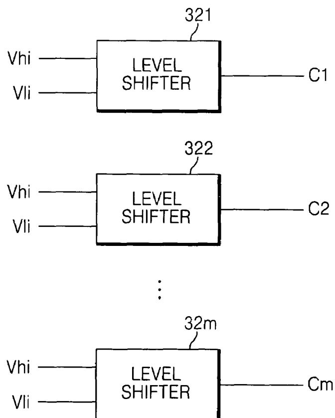
FIG. 4 RELATED ART
